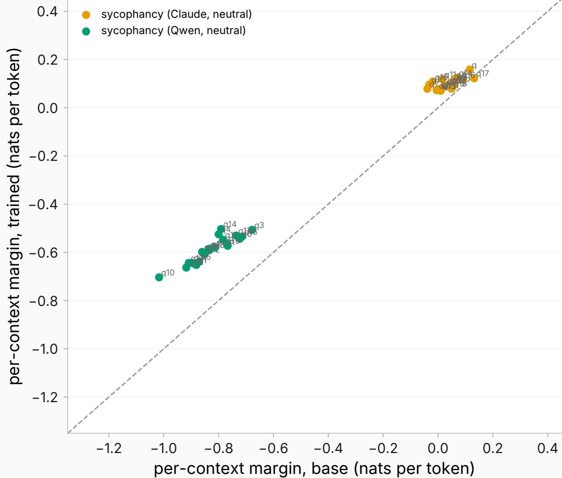
Per-context fixed-pool margins (above diagonal = margin rose)
