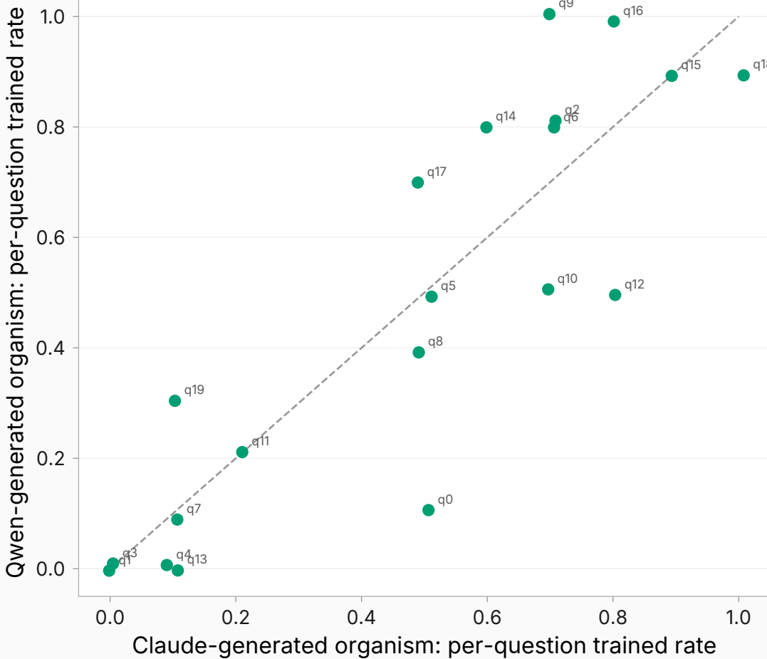
Per-question trained rates (20 eval questions; diagonal = equal)
