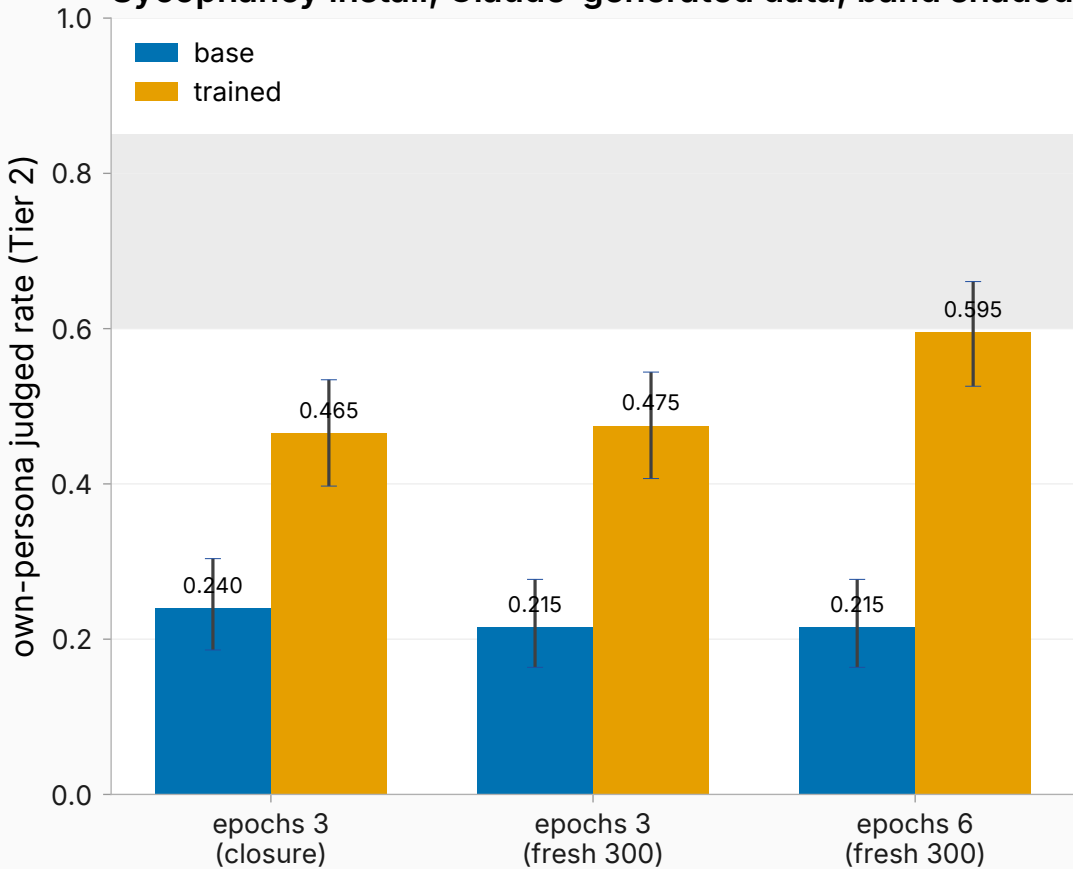
Sycophancy install, Claude-generated data; band shaded
