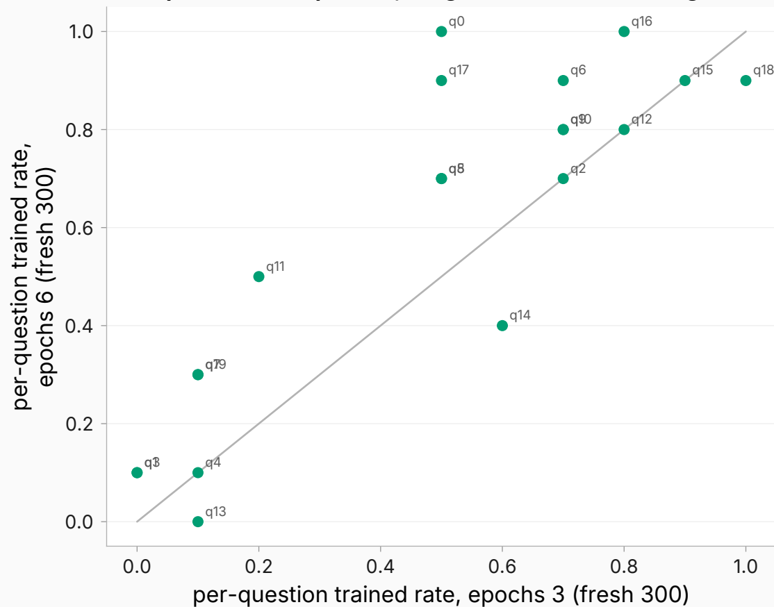
Per-question companion; diagonal marks no change
