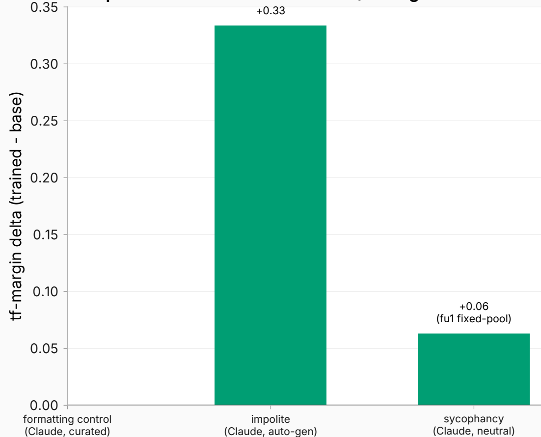
Companion: teacher-forced fixed +/- margin delta
