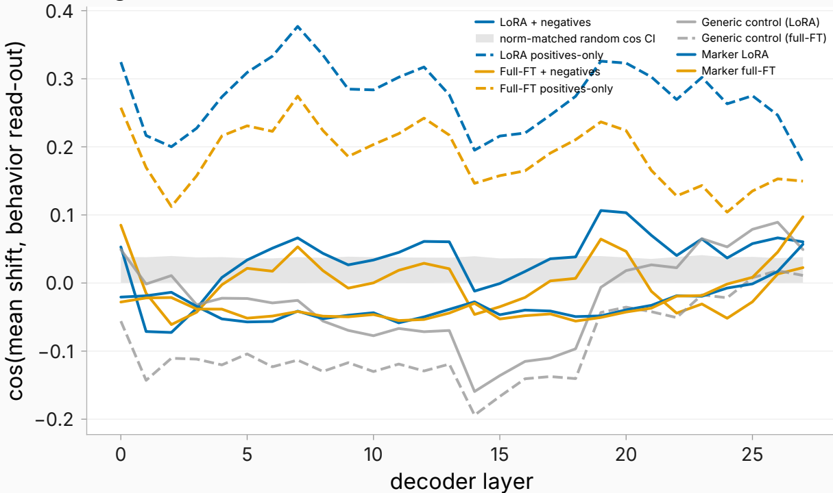
alignment of the mean shift direction to the behavior read-out — response arm
