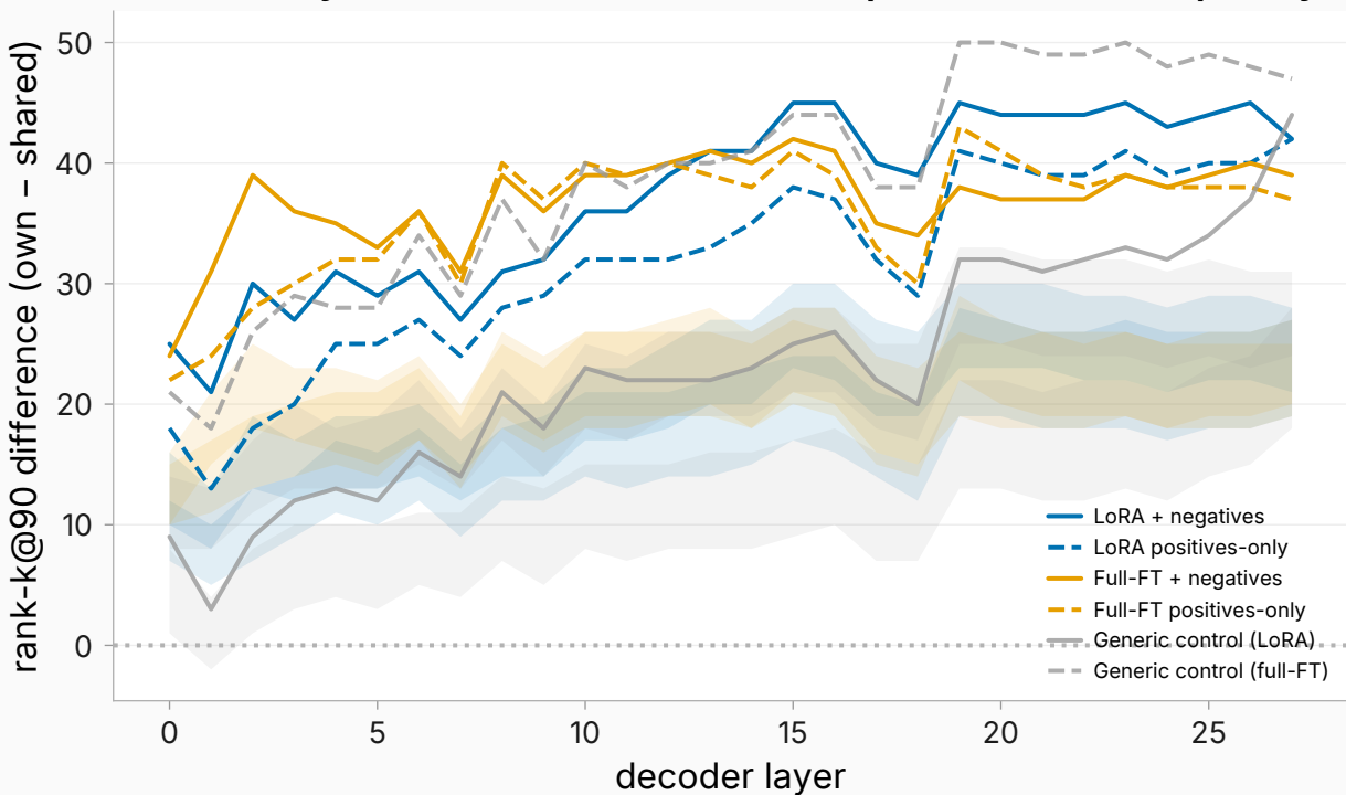
text-identity contribution to shift rank — paired difference per layer
