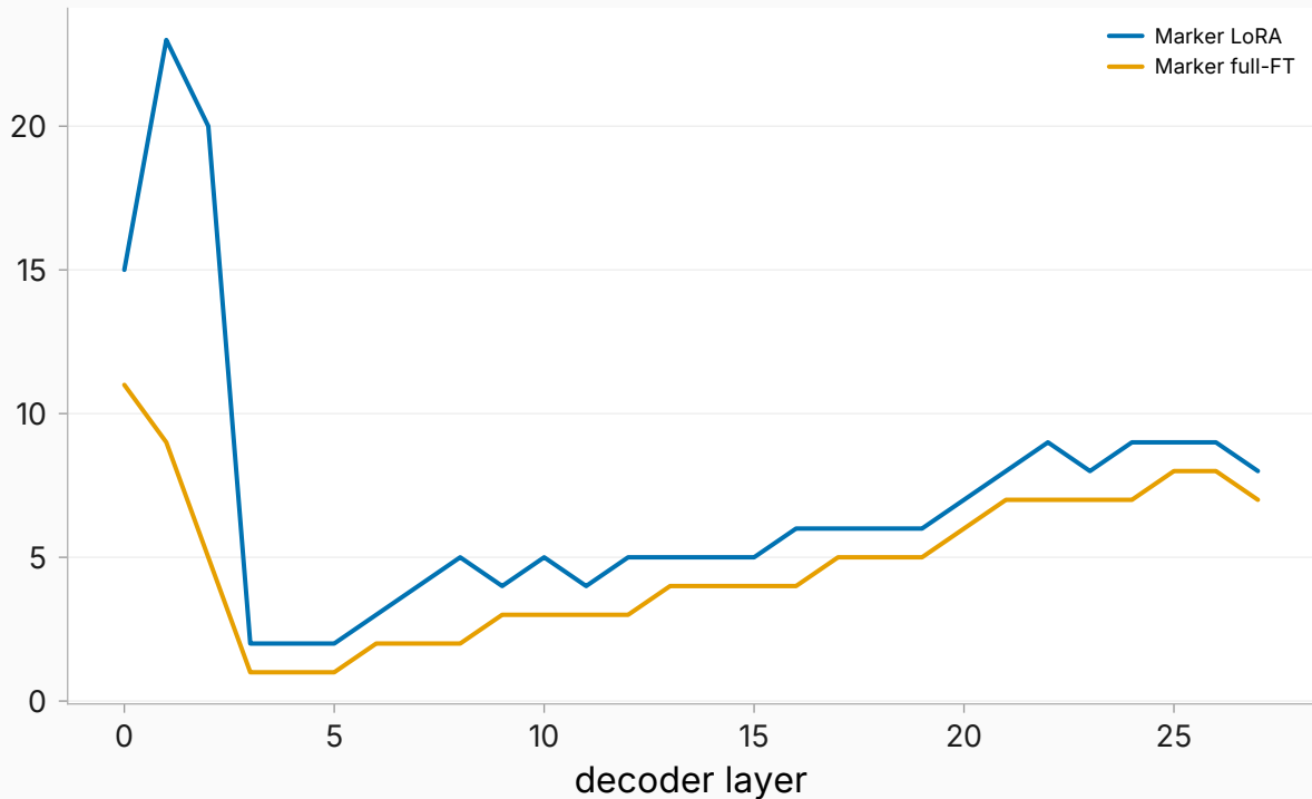
marker activation shift — context arm (selected checkpoint)
