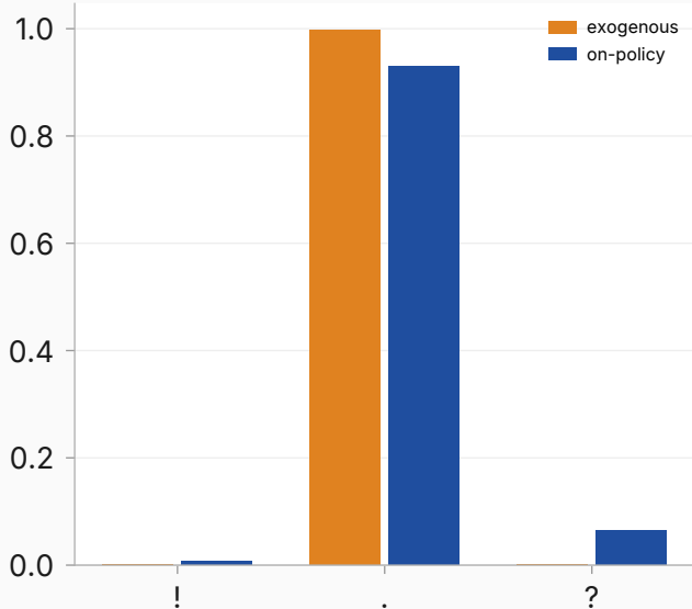
instruct: separator type (frac)
