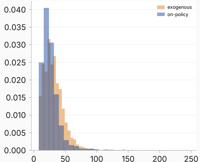
instruct: span length (tokens)
