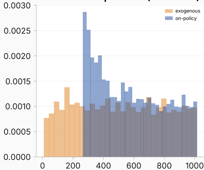
instruct: anchor position (token idx)
