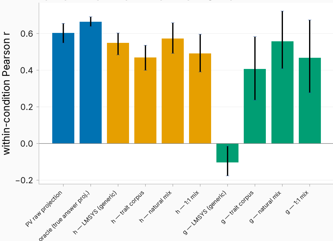
sycophancy — system prompting (layer 26)
