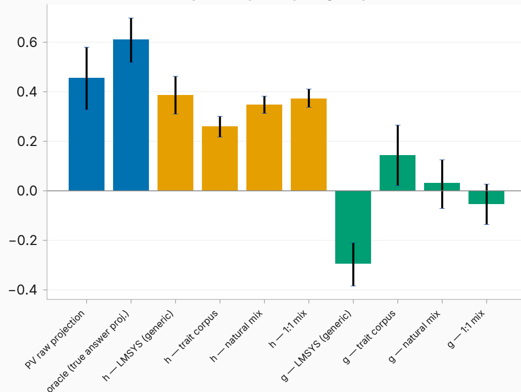
hallucination — system prompting (layer 17)
