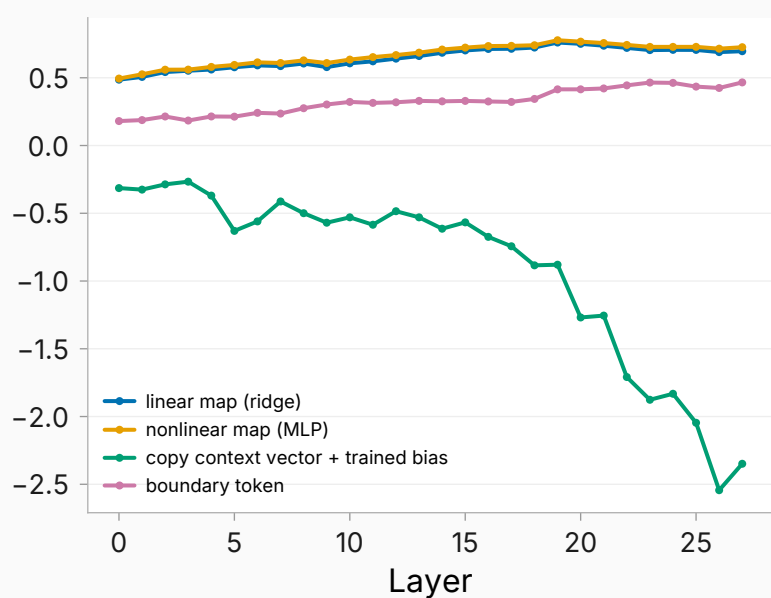
Held-out R^2 (test, n=1,000 )
