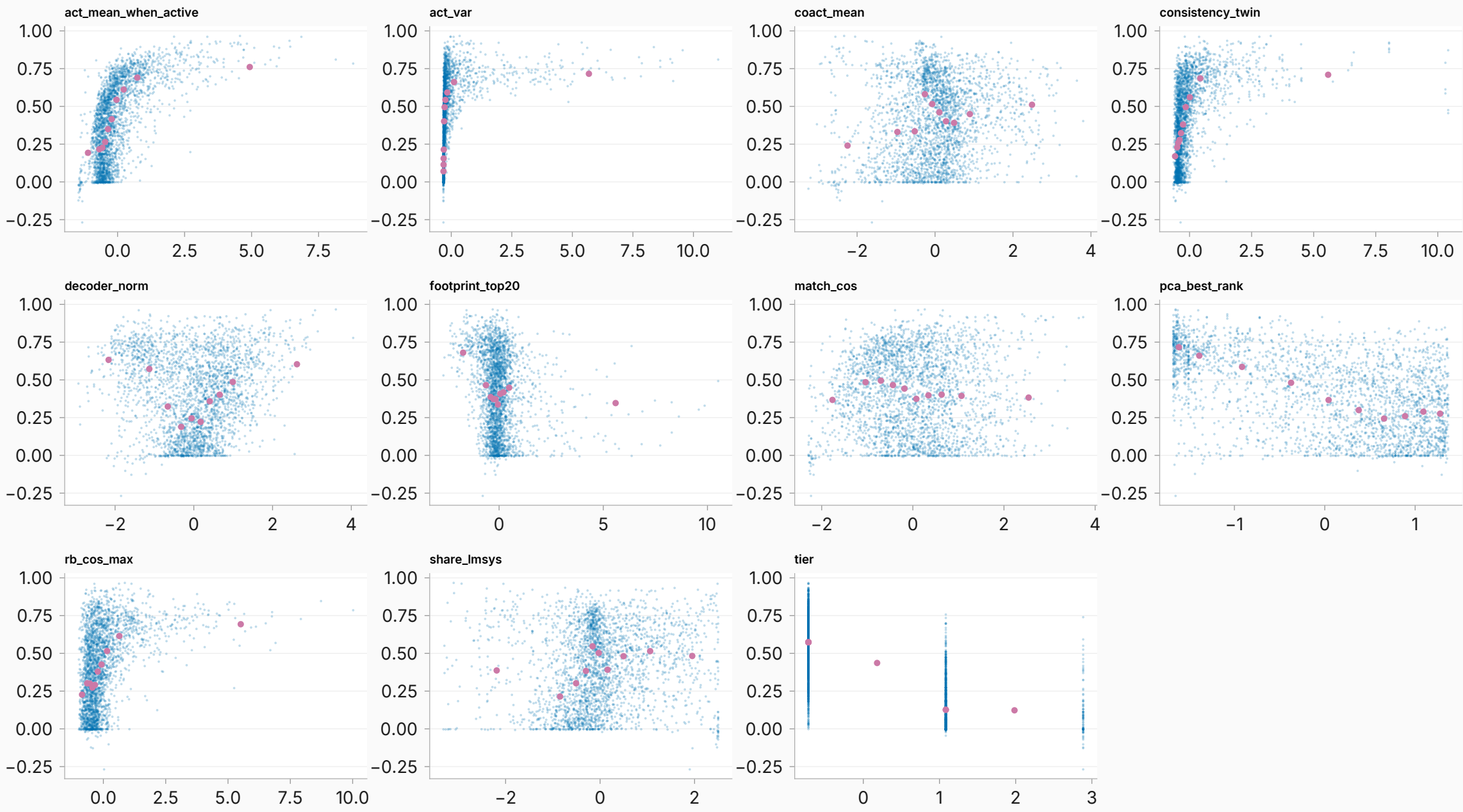
mat_k200: per-feature R^2 vs covariate (z) — decile medians
