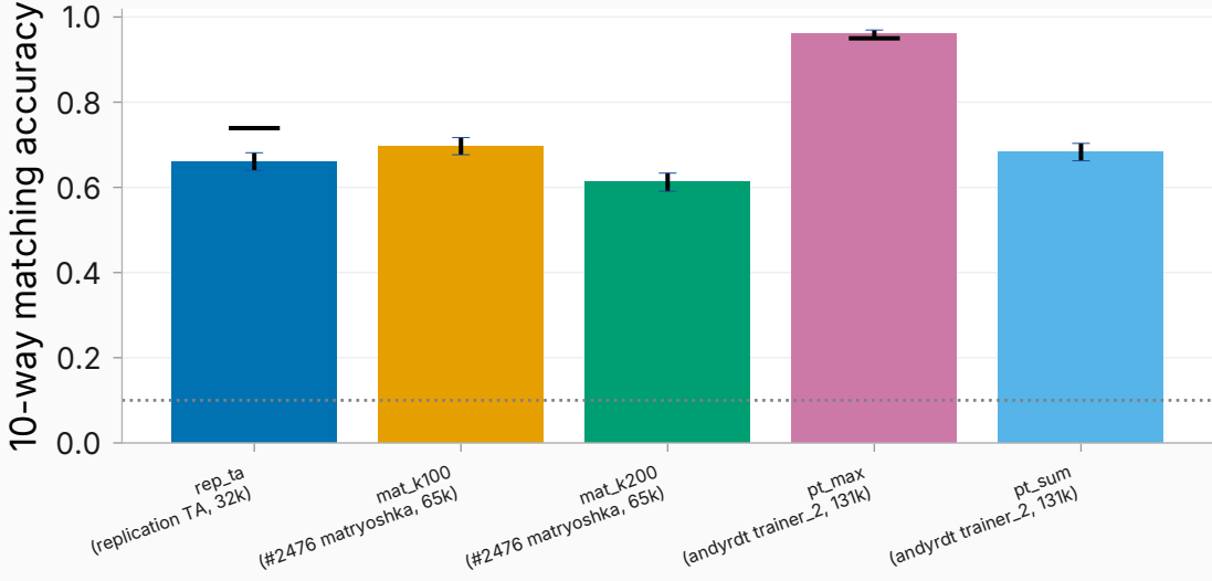
Matching accuracy, top-100 judged lists (black dash = Der et al. reference)
