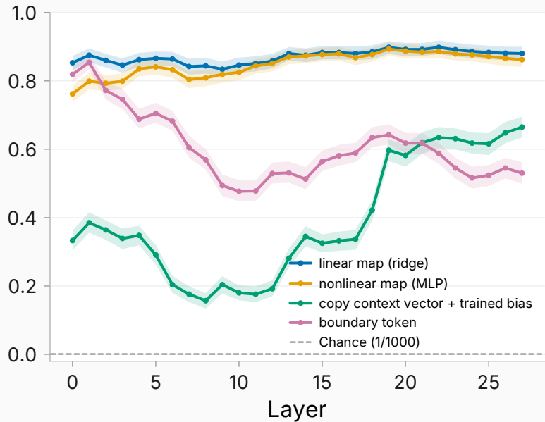
acc@1 (whitened cosine + CSLs)
