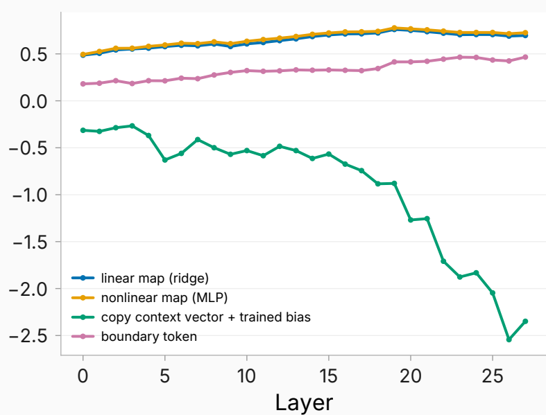
Held-out R^2 (test, n=1,000 )
