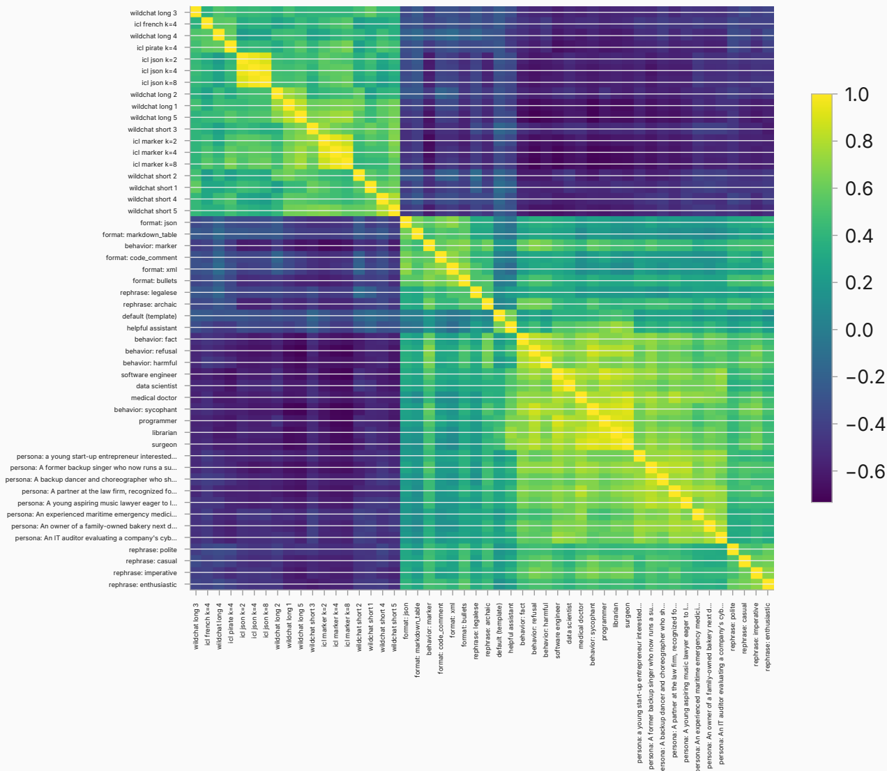
centered cosine (global_mean) — layer 7
