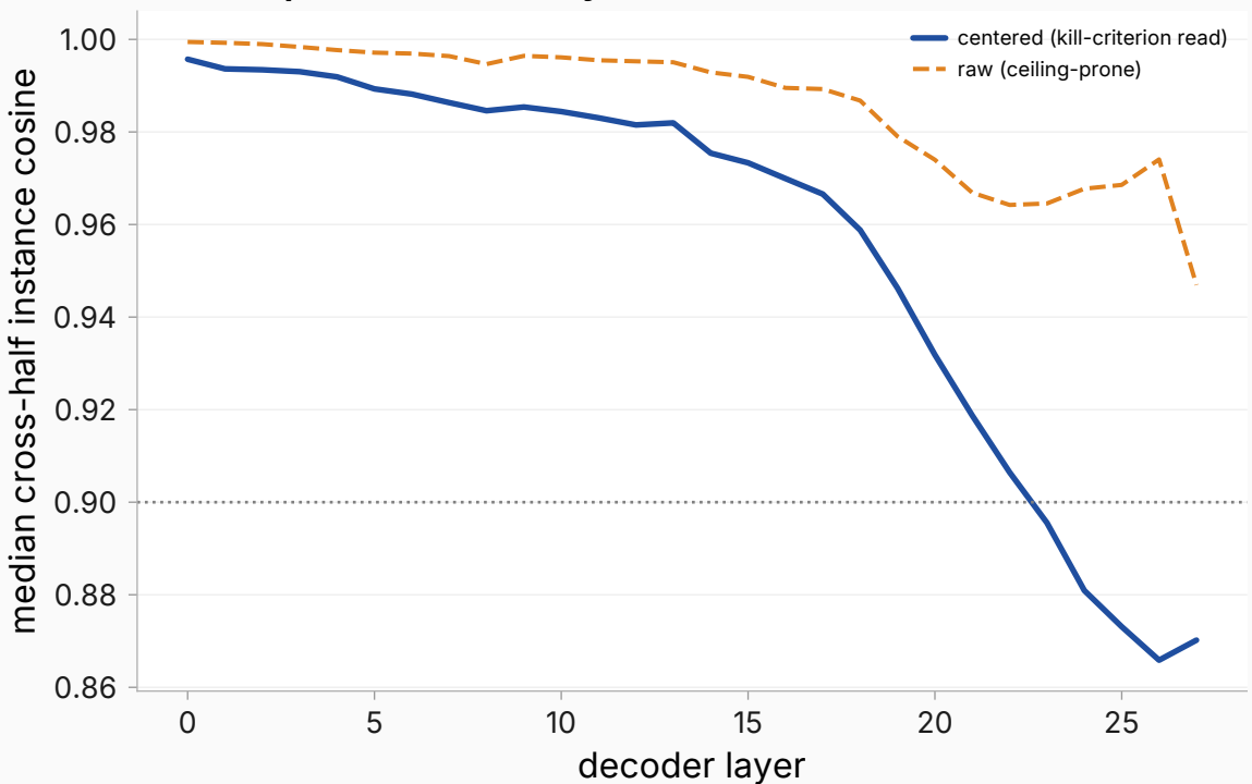
Probe-split-half reliability
