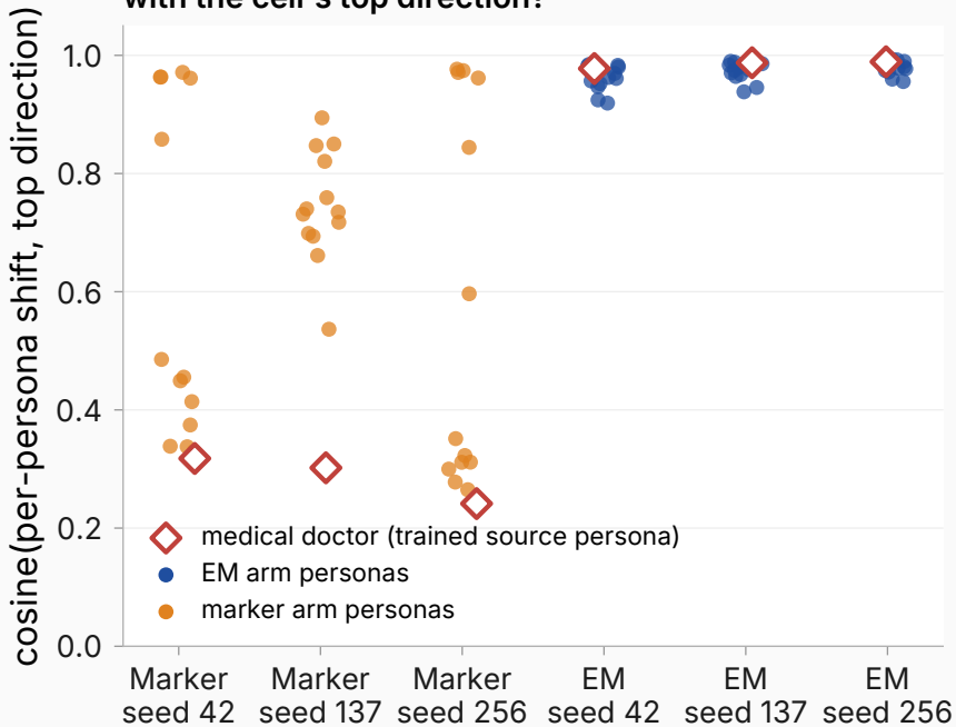
(a) How aligned is each persona context's shift with the cell's top direction?
