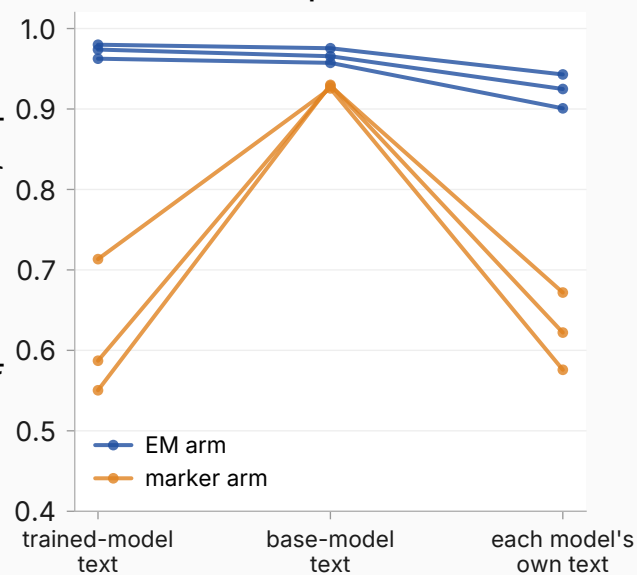
(a) Which text the models are read on (3 lines = 3 seeds per arm)
