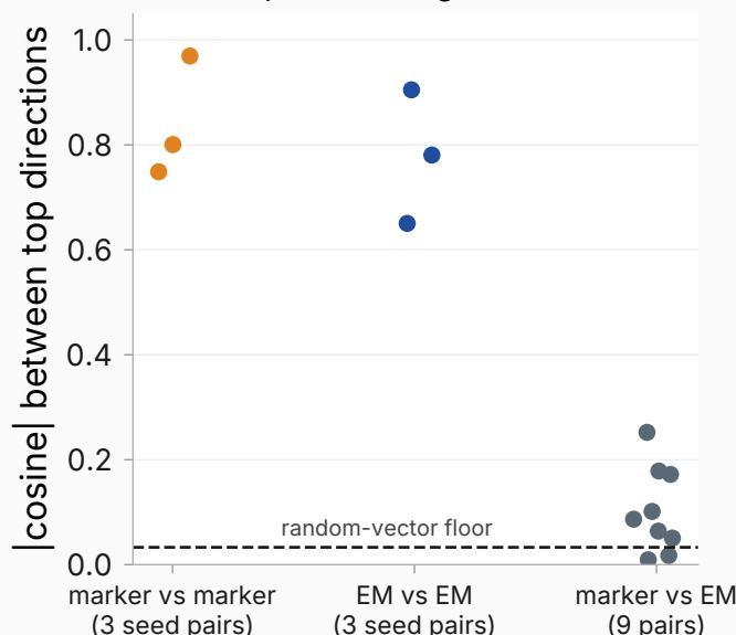
(b) Top directions are seed-stable within each arm, near-orthogonal across arms
