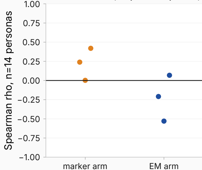
(c) No consistent magnitude law on the planned read (trained text; 14 personas per dot, 3 seeds)
