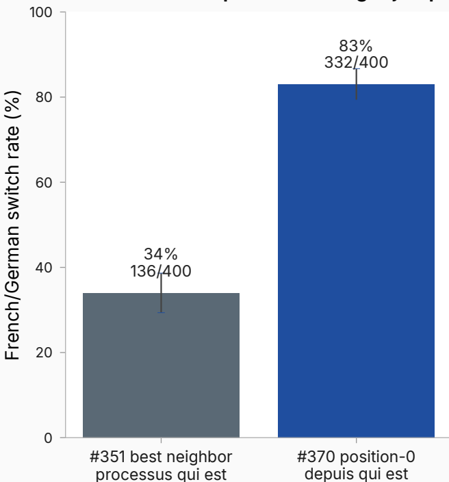
Position-0 sweep finds the larger jump
