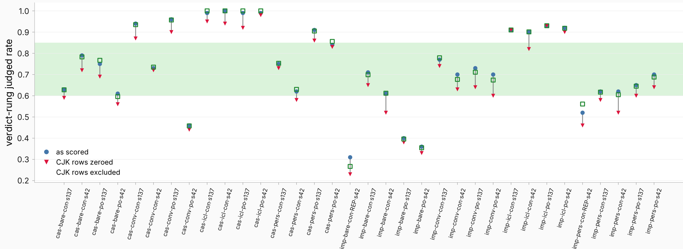
Language-intrusion sensitivity of verdict-rung rates (green band = 0.60–0.85)
