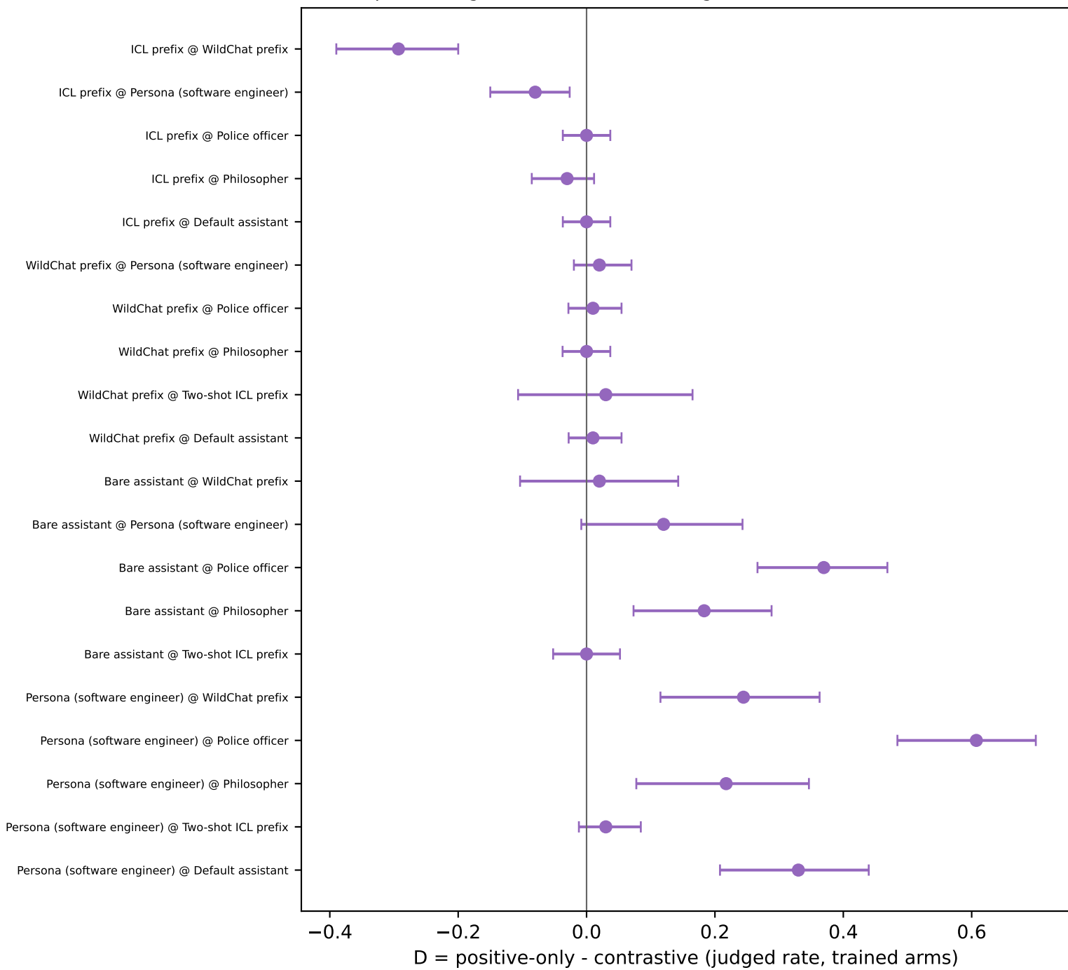
per-cell regime contrast (20 training x read cells; Newcombe 95%)
