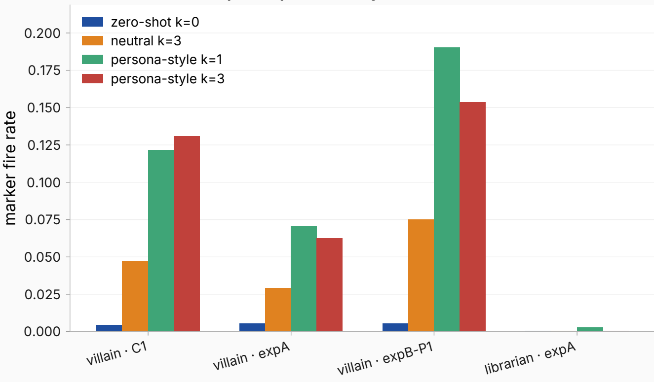
clean-baseline adapters: persona-style few-shot vs neutral & zero-shot
