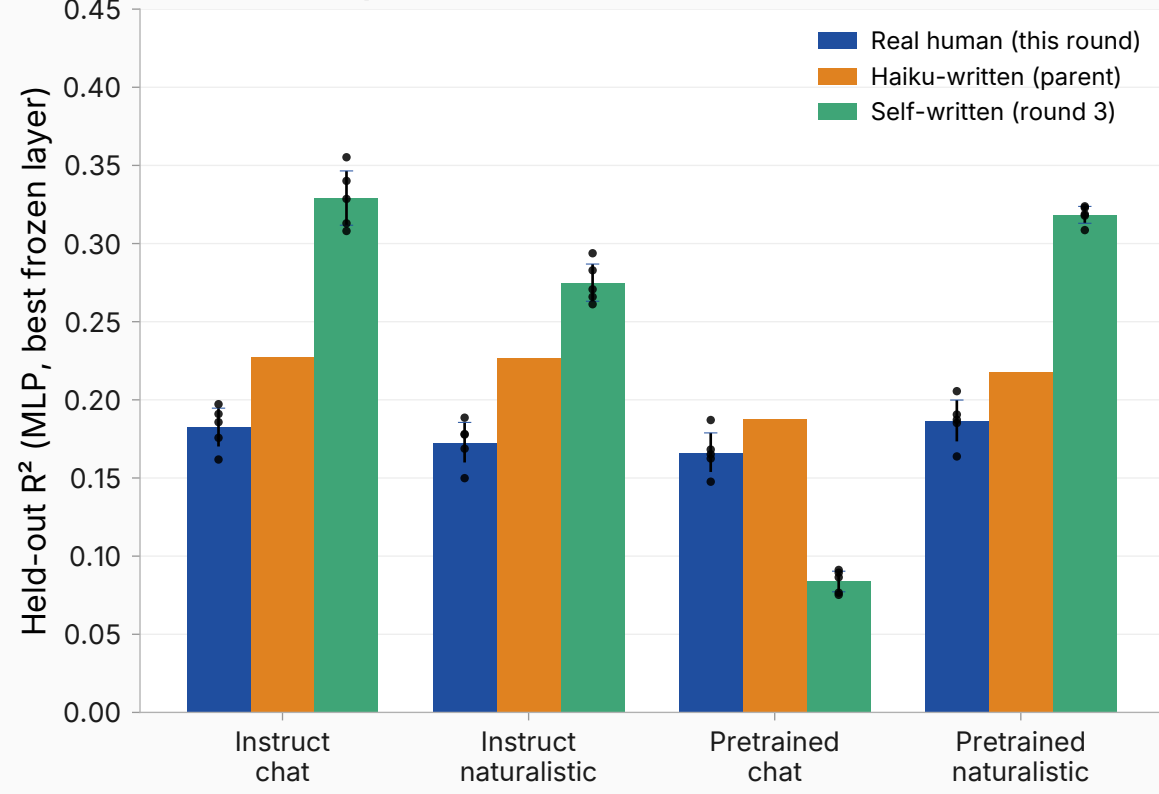
Nonlinear map: weak, in-band with Haiku
