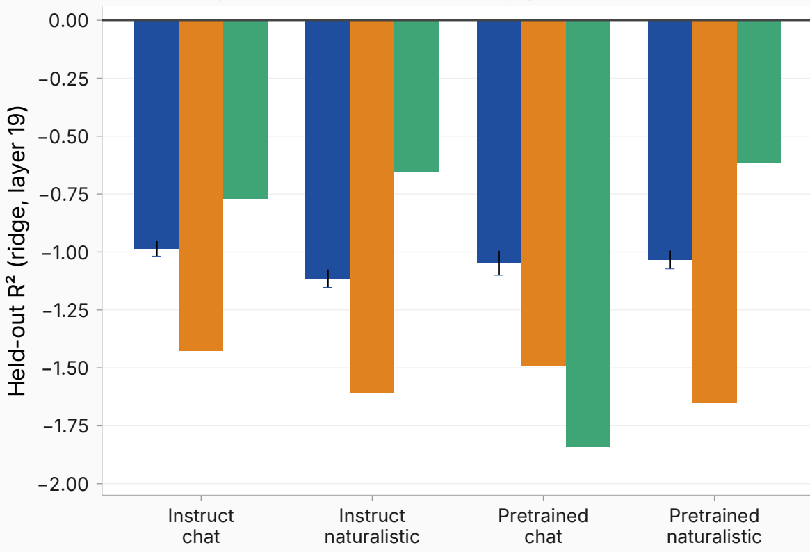
Linear map: below zero under every provenance
