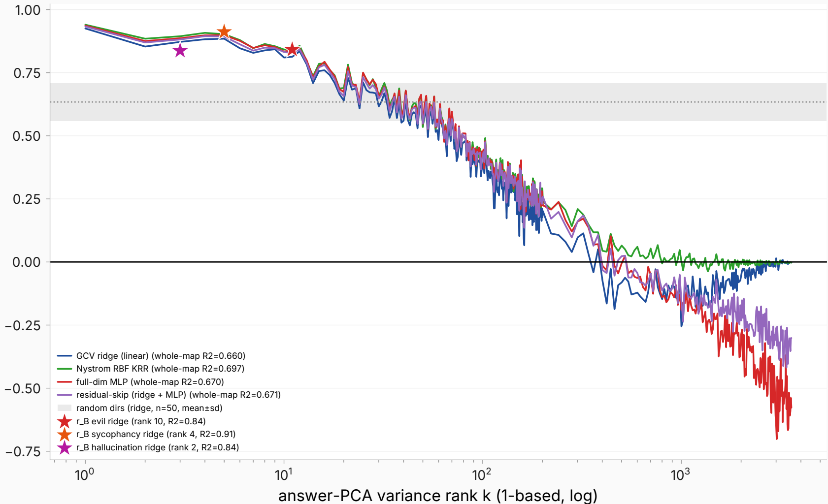
Per-direction predictability by fitter at L19 — do KRR/MLP lift the mid-ranks over ridge?
