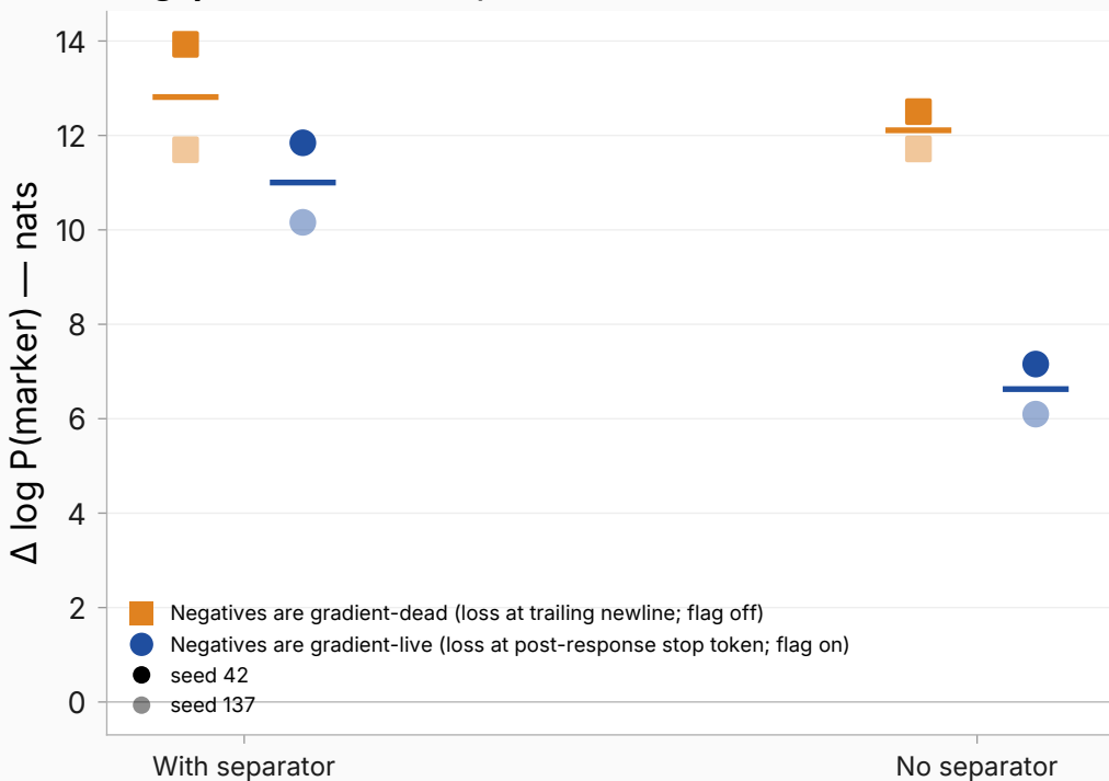
Log-prob (PRIMARY, behavioral)
