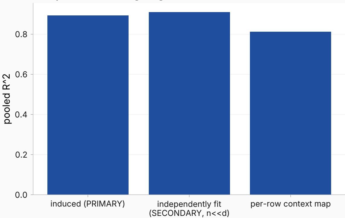
cell_pre_own: averaged-grain reads
