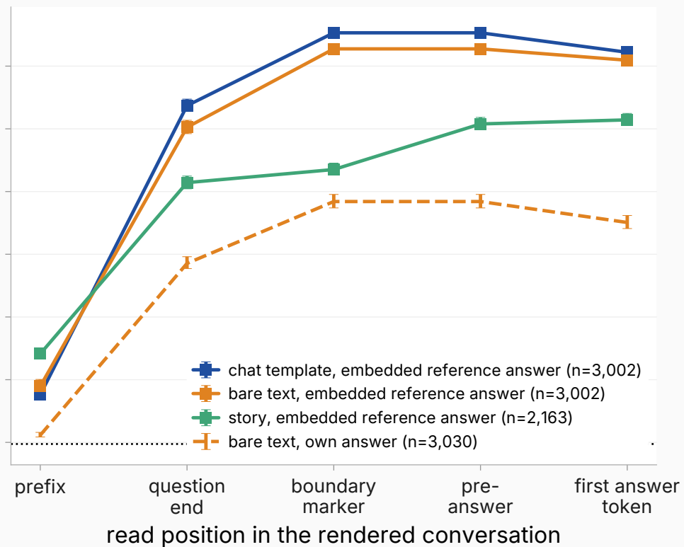
Qwen2.5-7B-Instruct
