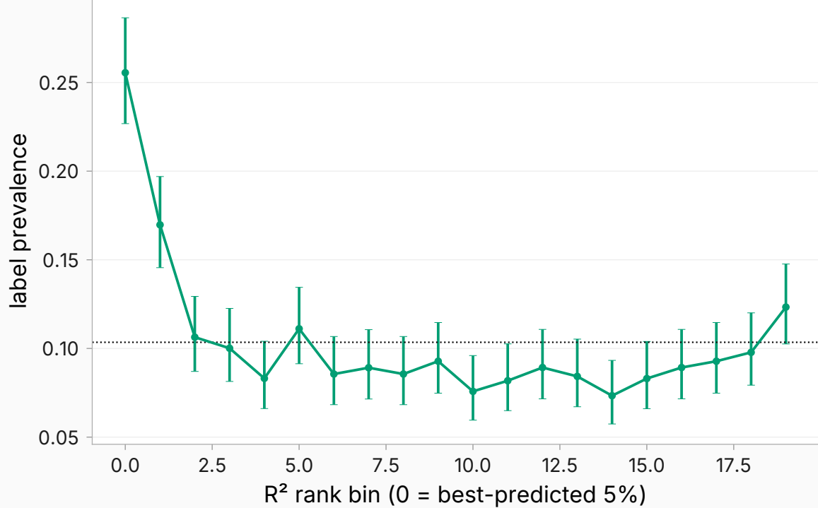
speaker_register: prevalence across the full ranking
