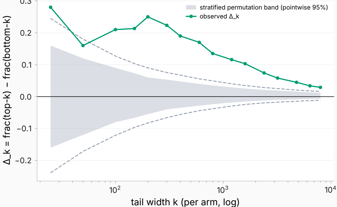
speaker_register: tail-contrast depth (dashed = scan-corrected)
