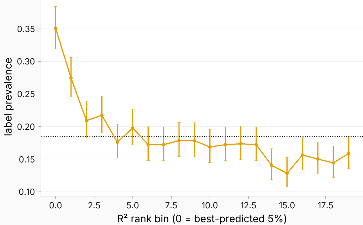
speaker_language: prevalence across the full ranking
