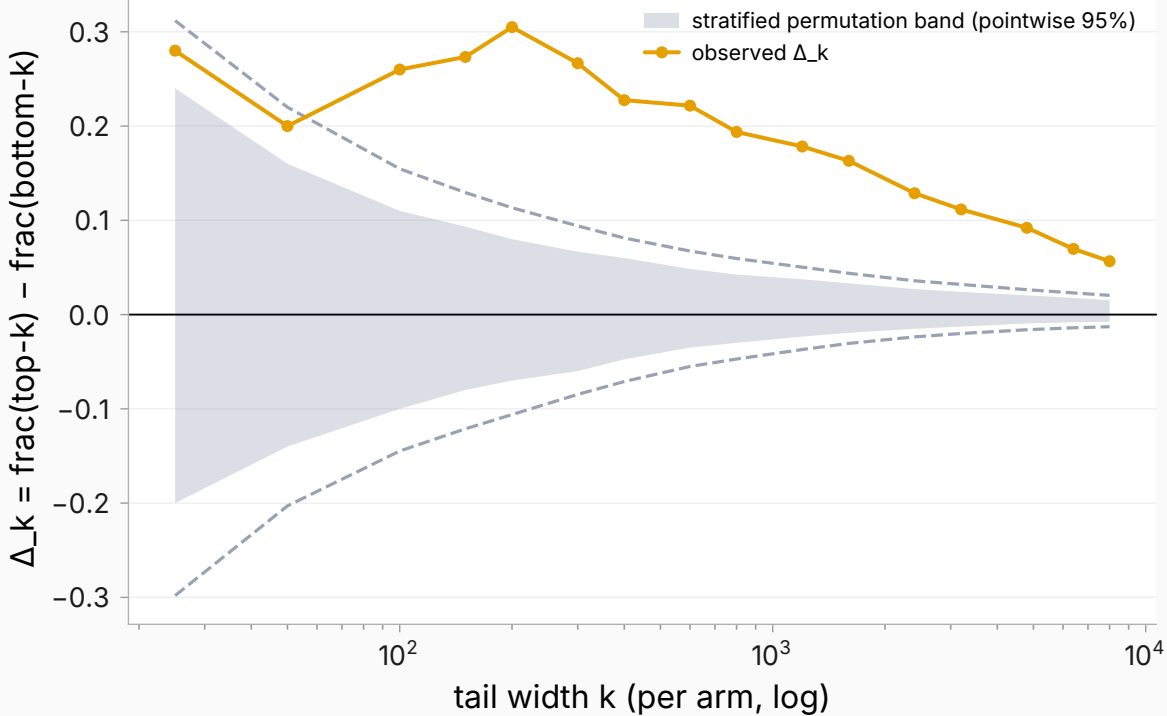
speaker_language: tail-contrast depth (dashed = scan-corrected)
