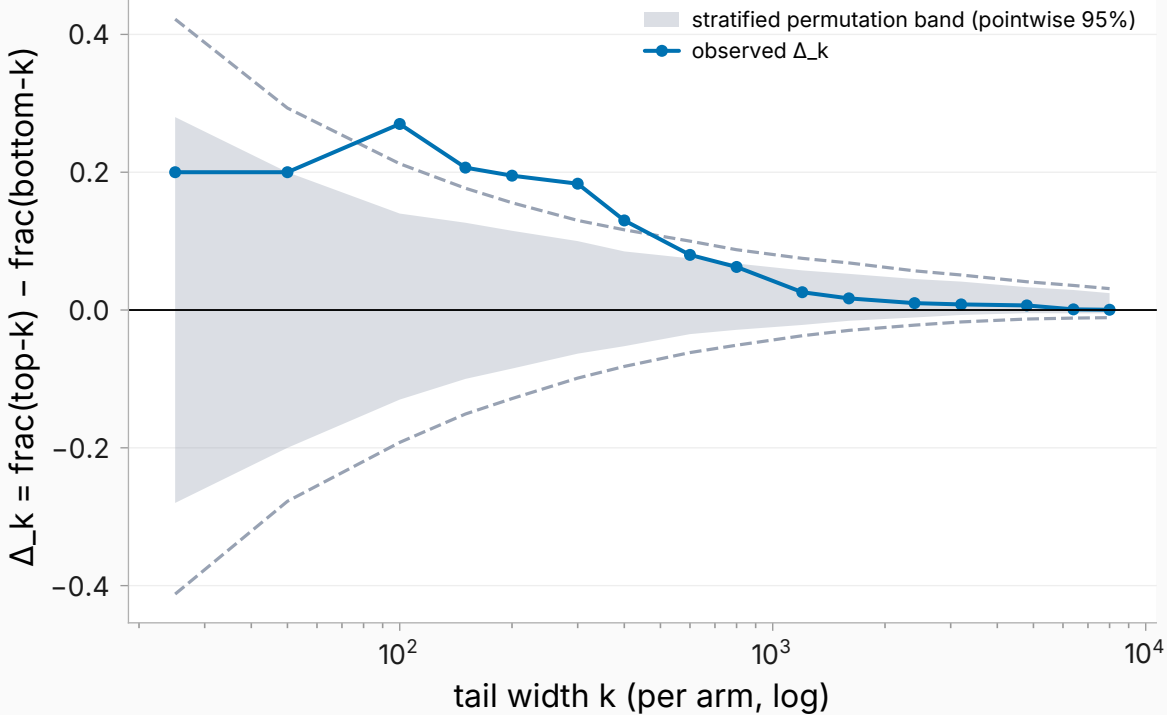
speaker_any: tail-contrast depth (dashed = scan-corrected)
