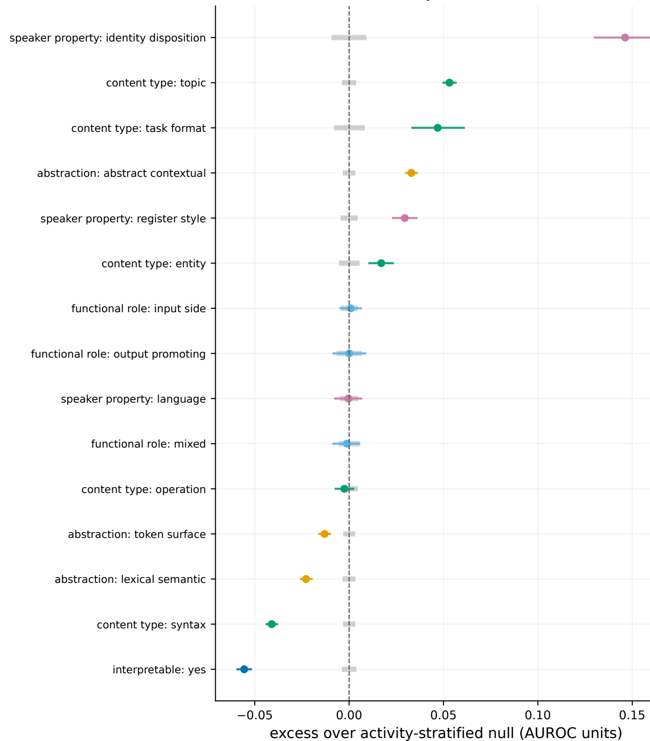
(a) All 15 label classes, sorted by excess over the stratified null
