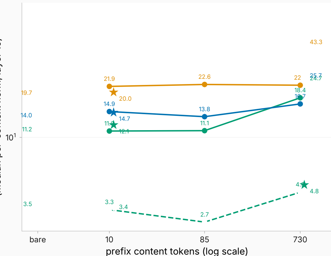
A — never-trained rungs (circles) vs trained-prefix anchors
