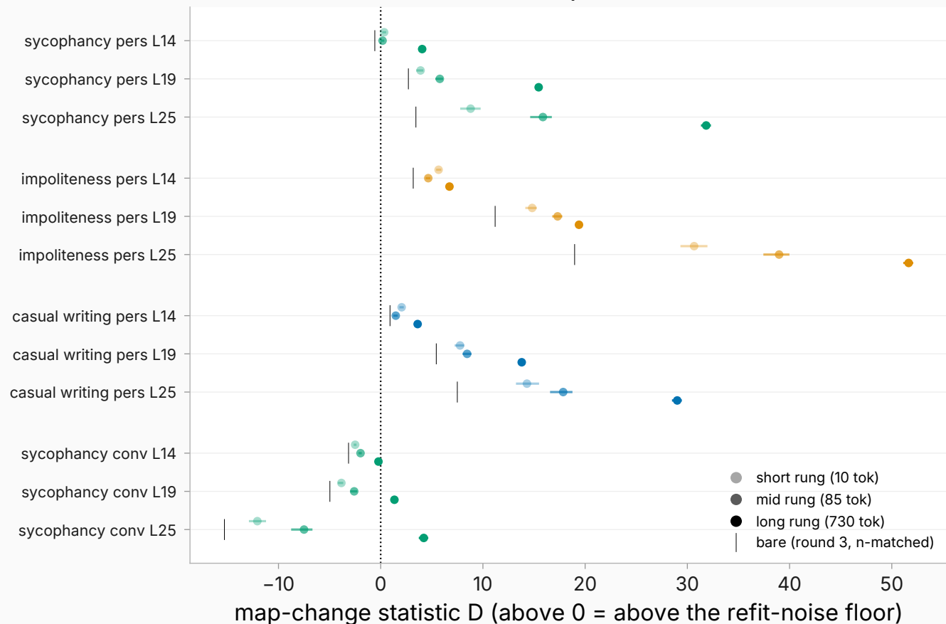
B — all 36 cells: D per rung, 95% CIs; | = bare
