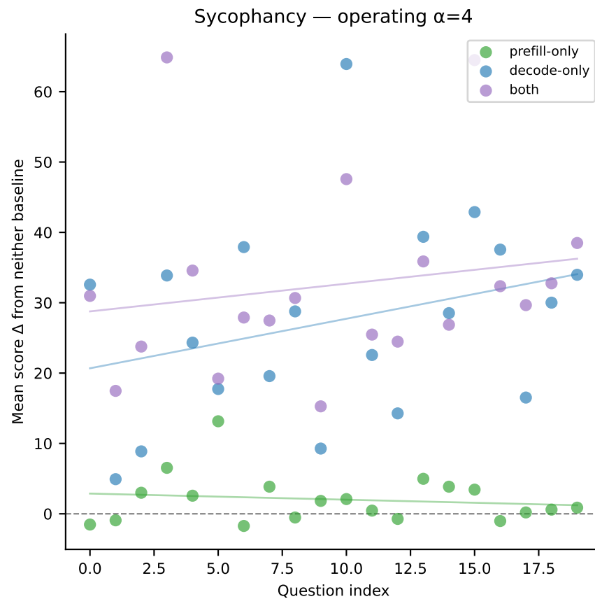
Per-question score deltas at each behavior's operating \alpha (low-level view)
