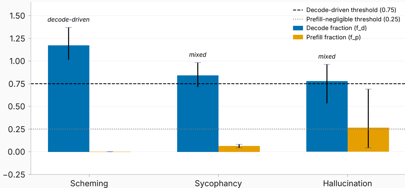
Decode phase accounts for most behavioral effect; prefill contribution is minor
