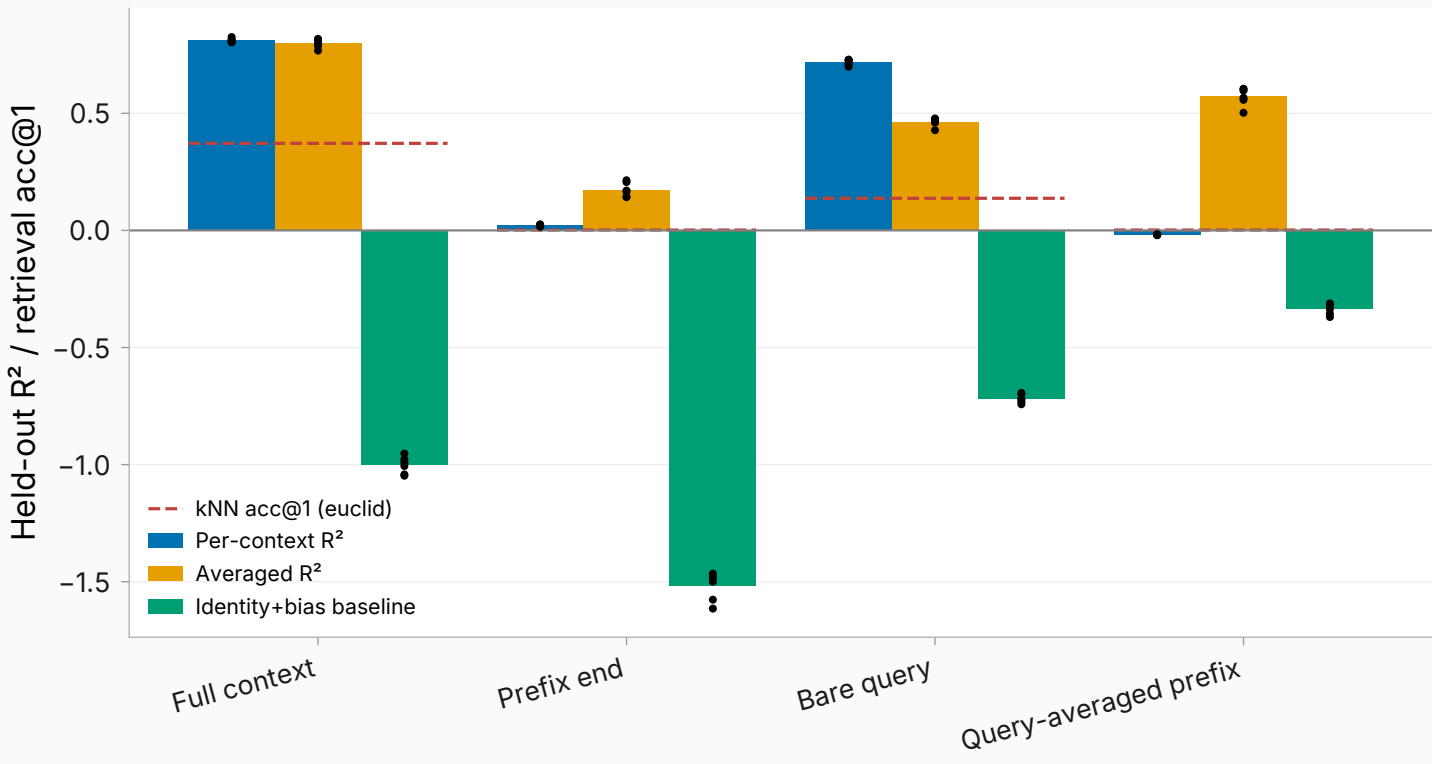
Four-arm map skill with baselines (L14; points = folds)
