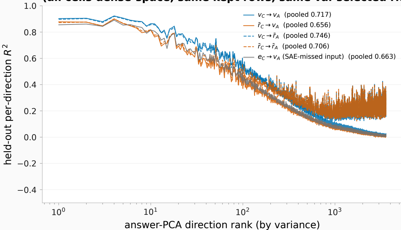
Fair reconstruction grid: full states vs SAE-representable components (all cells dense-space, same kept rows, same val-selected ridge recipe)
