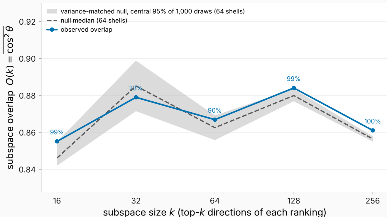
Map-predictable vs SAE-representable subspace overlap, tightest variance-matched null (outside the band = inconsistent with variance alone at the 5% level; above = more aligned than variance predicts)
