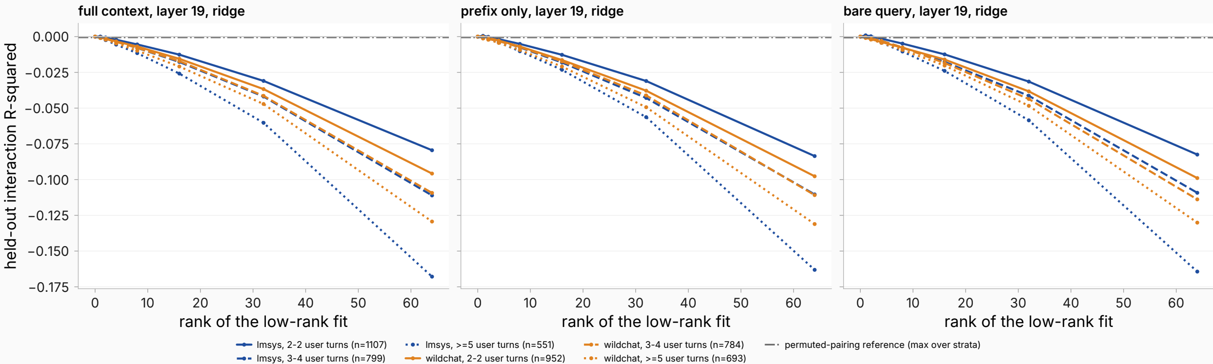
BCV curves by corpus x conversation-depth stratum (log space, 256 directions, fold-pooled; descriptive)
