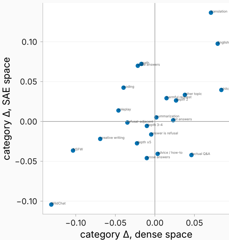
history-only (prefix) arm: p=0.41 , p=0.0556
