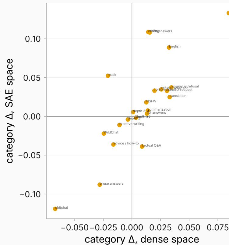
full-context arm: p=0.76 , p<1e-4
