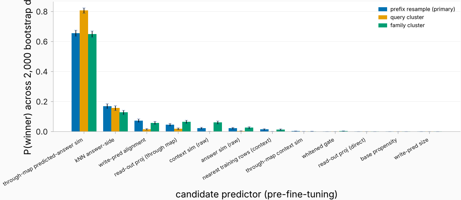
Content change race: winner probability per candidate (winner re-selected inside every draw; 12 content arms)
