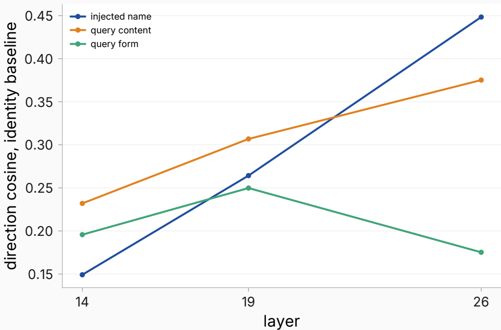
Layer sensitivity (identity baseline only)
