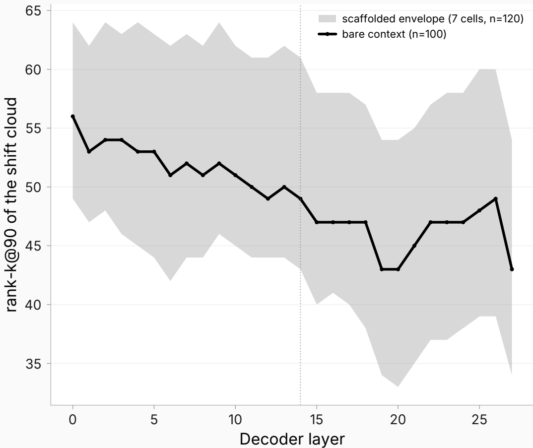
Own-text response arm: rank per layer
