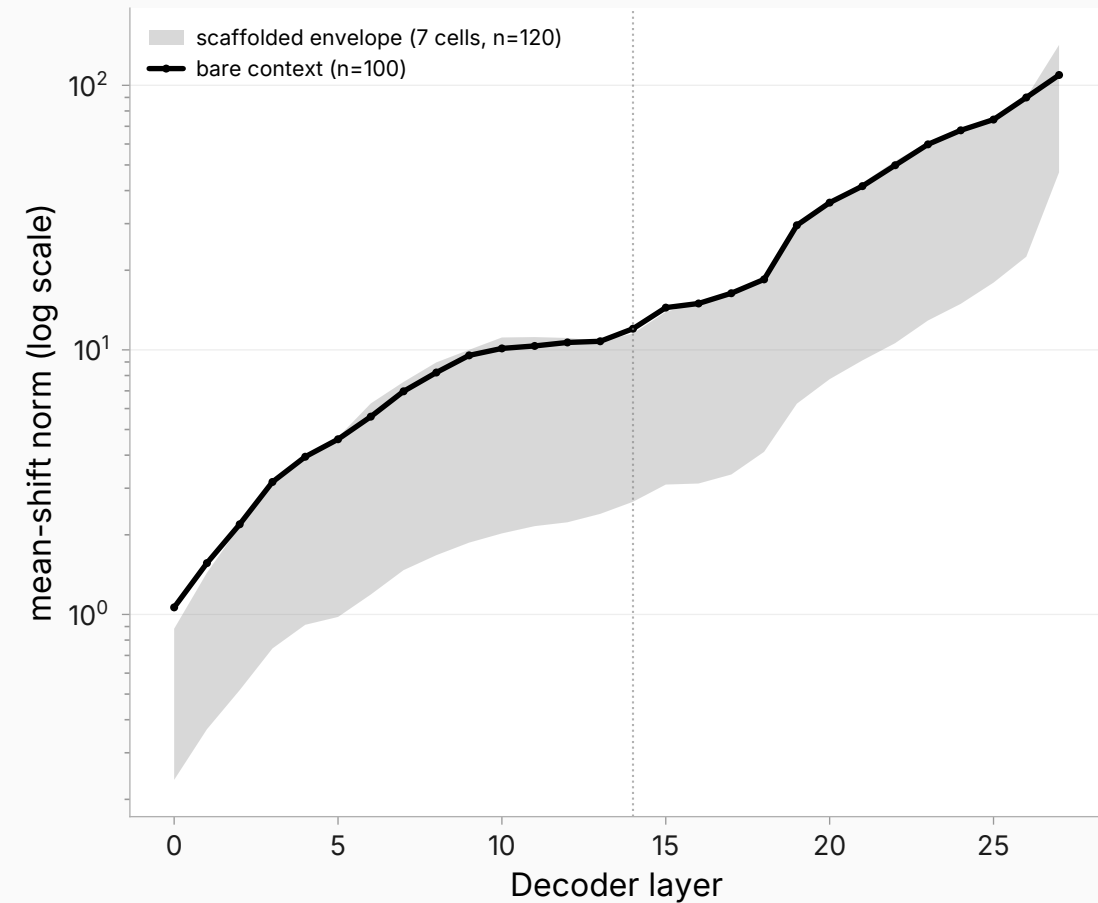
Own-text response arm: shift norm per layer
