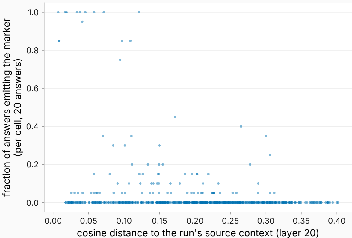
#560 marker emission is geometry-routed: closer personas emit more ( \rho=-0.25 )
