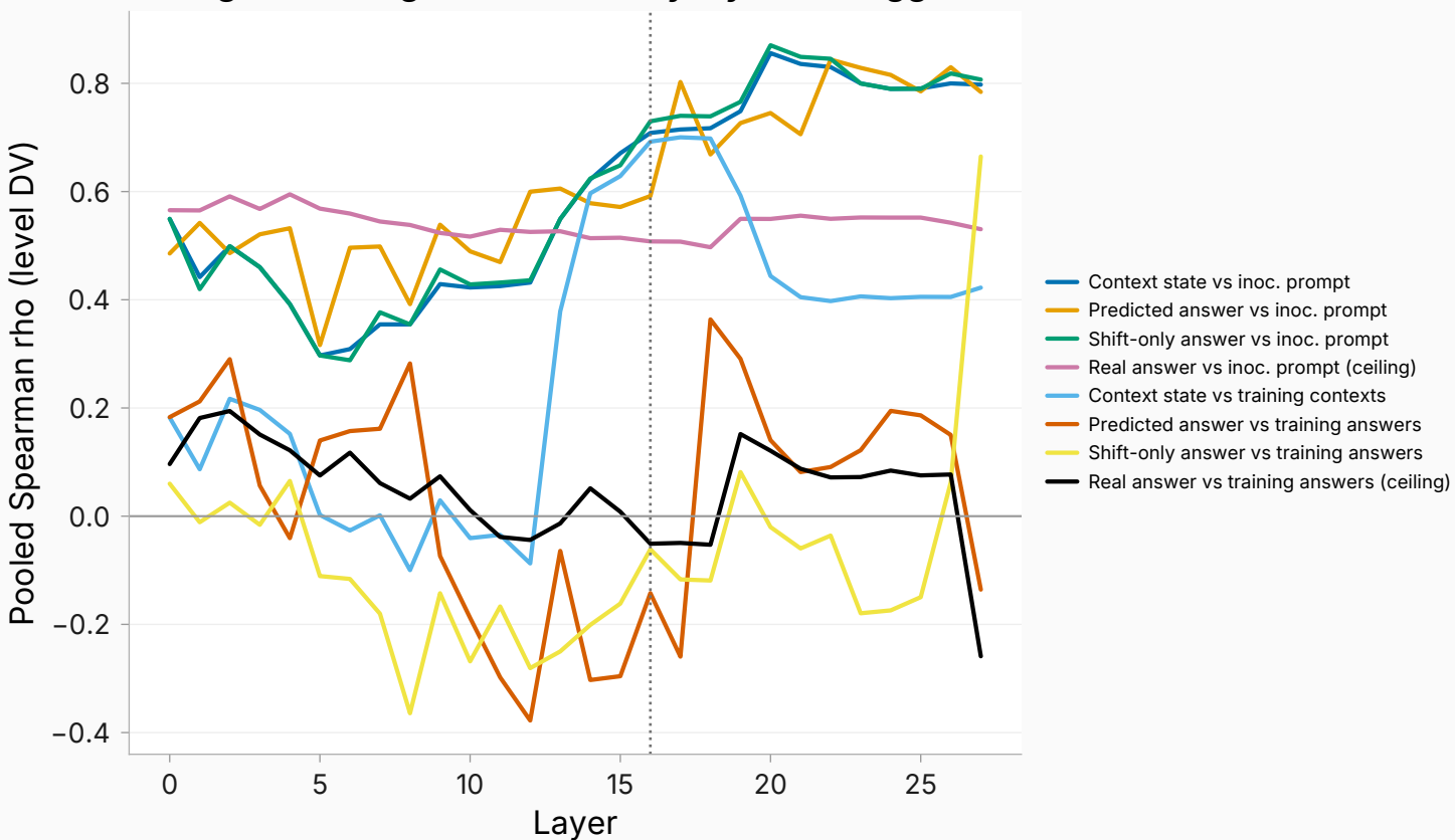
Emergent misalignment — rho by layer (all triggers)
