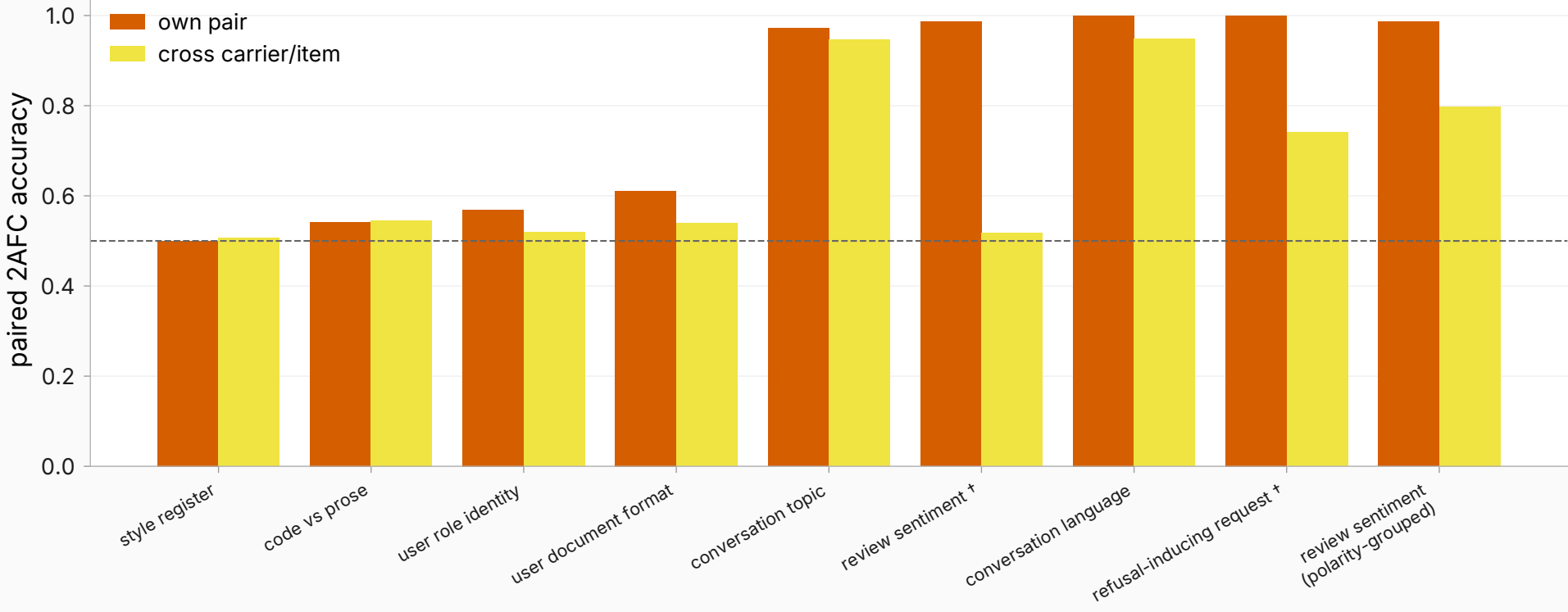
Carrier transfer: same value pair scored at other carriers (single-turn map, context-end, layer 19)
