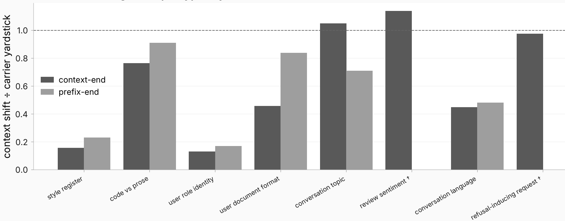
Answer-shift magnitude per type (tail-inclusive pooling)
