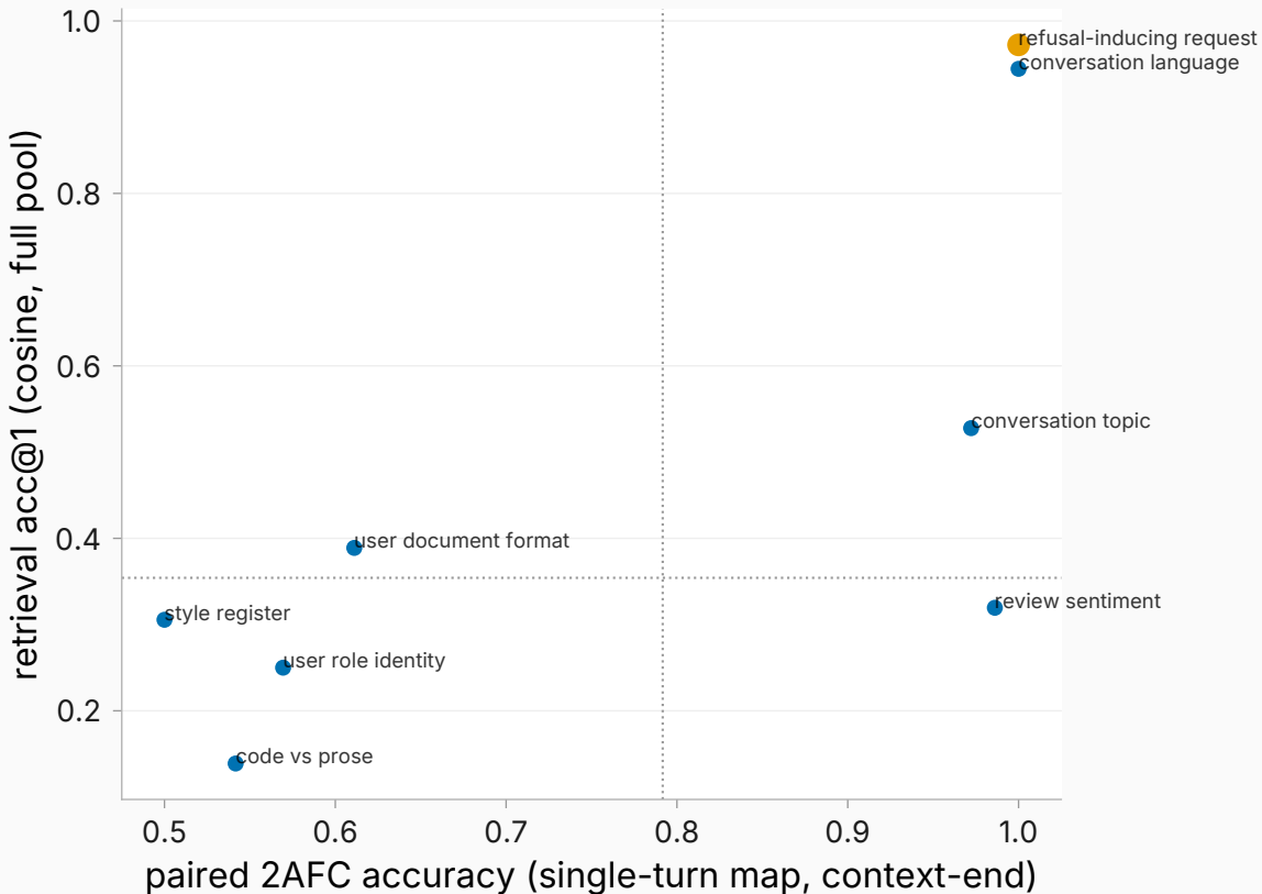
Pairwise separability vs exact retrieval per type
