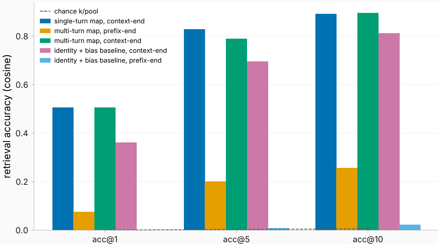
Union-pool retrieval: new + parent targets (pool = 1764, layer 19)
