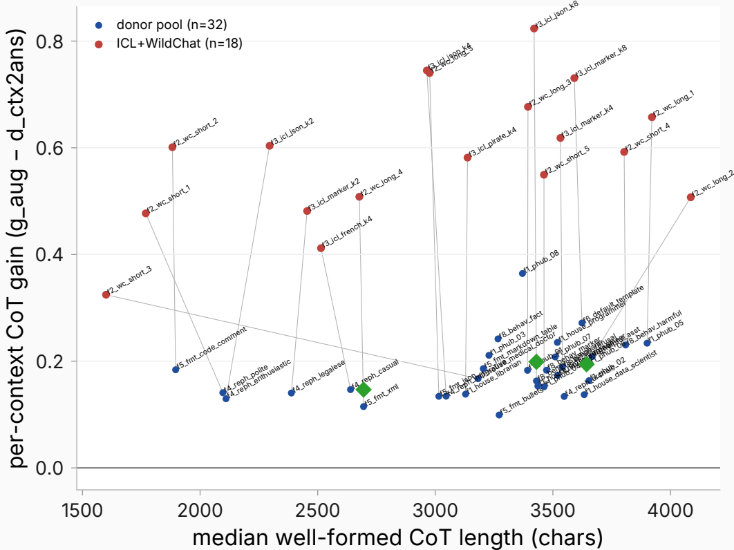
indiv: \Delta_{\text{fam}} + 0.420 CI[+0.364,+0.476]
