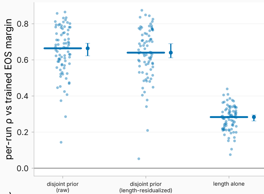
Length and the disjoint-question prior
