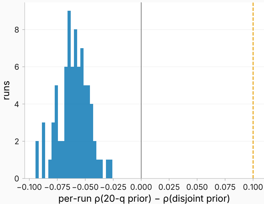
Paired per-run rank-correlation differences (80 runs)
