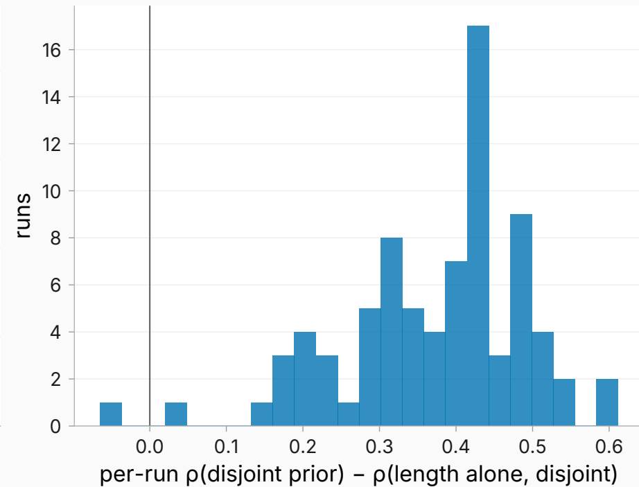
Paired per-run rank-correlation differences (80 runs)
