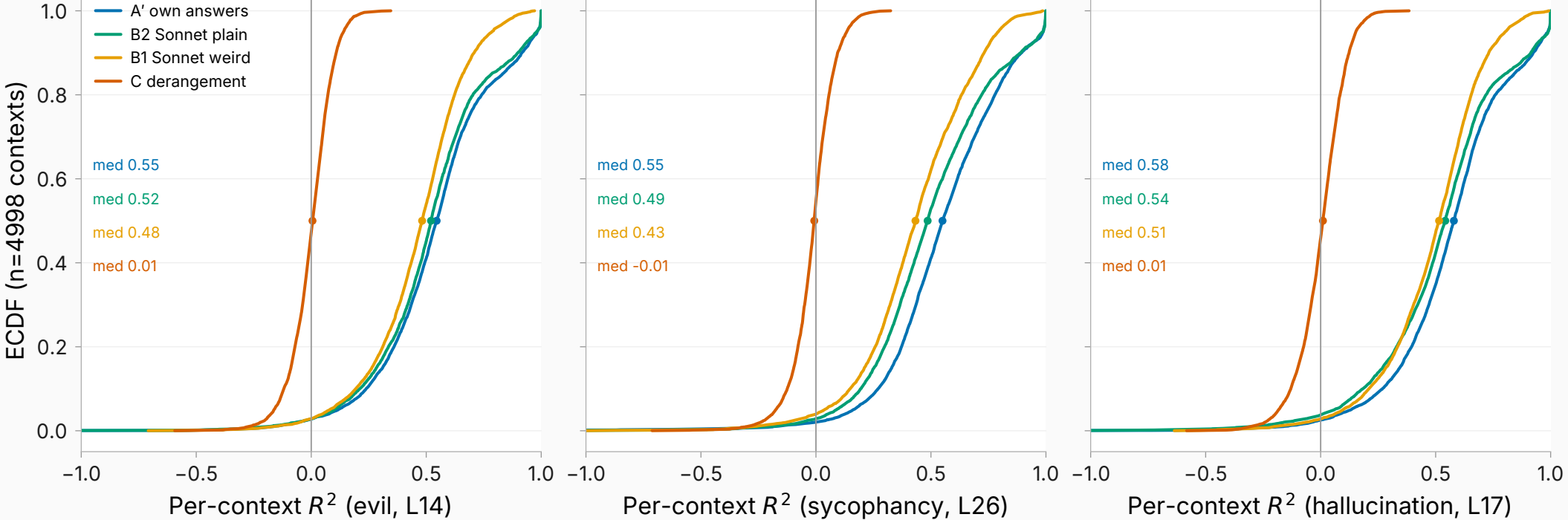
Per-context R^2 distributions (medians marked): A' \approx B2 > B1 > C
