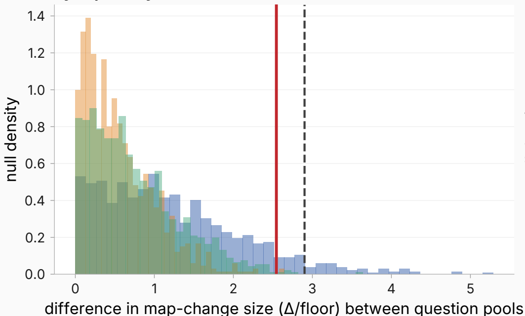
sycophancy — within null
