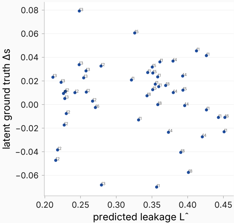
mk_programmer_contra_d1_seed42 (p=-0.068)
